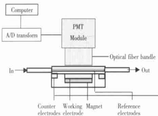
Fig. 2 A diagram of the essential components of the instrument
