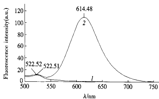
Fig. 1 Fluorescence spectrum of [Ru(bpy)_3]^{2+}
