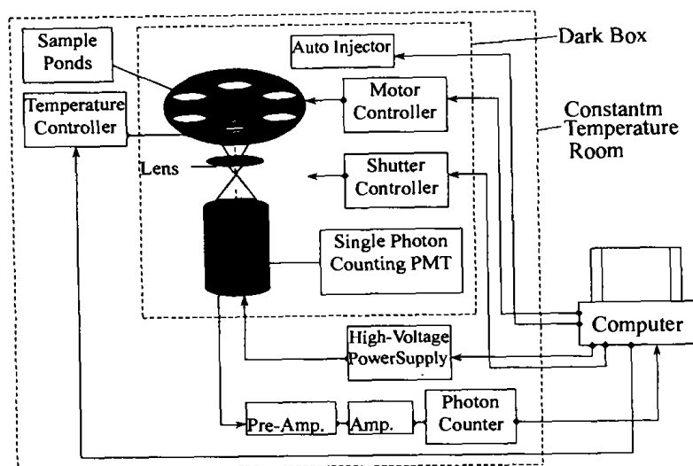
Figure 1 The schematic of single photon counting system
